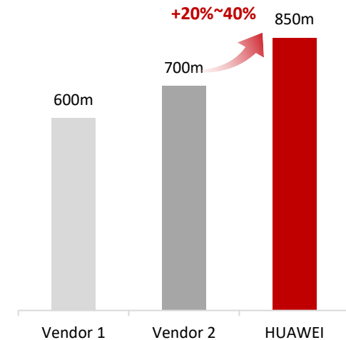
N78 Coverage (Distance)
