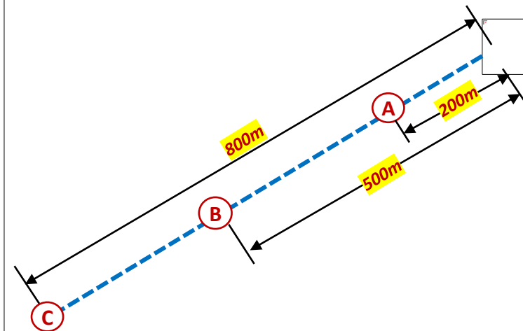
Near/Mid/Far Point Testing
